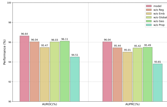
Fig. 3 Ablation study of GCFH-MDA.
