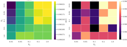
Fig. 5 Loss weight sensitivity analysis of GCFH-MDA
