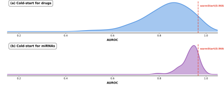
Fig. 6 Cold-start performance of GCFH-MDA
