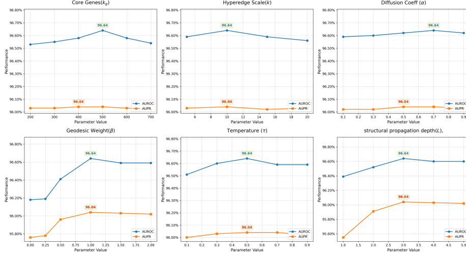
Fig. 4 Hyperparameter sensitivity analysis of GCFH-MDA.
